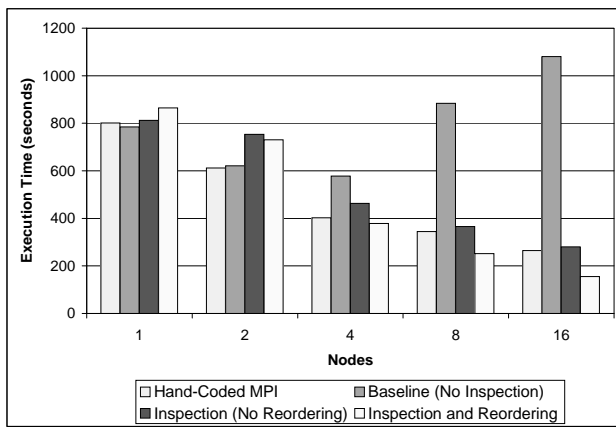
Figure 7. Performance of Equake .
